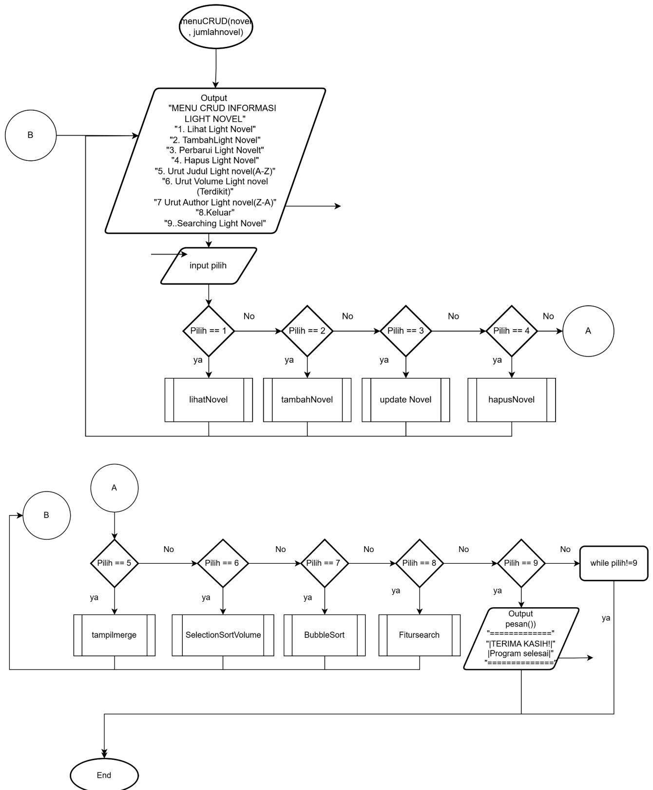
Gambar 1.3 Flowchart menu CRUD
